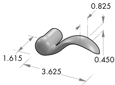
L-95RH Little Beaver Tail lever. Right hand.
