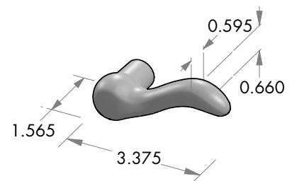
L-93RH Chubster lever. Right hand.
