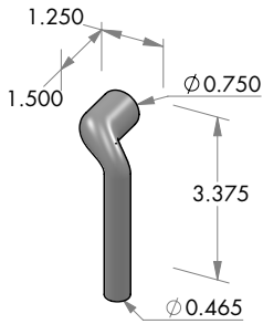
L-12OH-RH Tiny Tube lever. Right hand.
