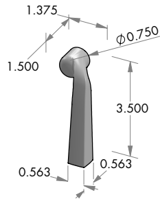
L-96OHRH Squarelet lever. Right hand.
