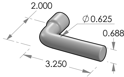
L-12 Tiny Tube lever.
