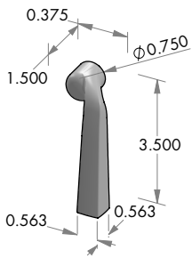
L-96OHLH Squarelet lever. Left hand.
