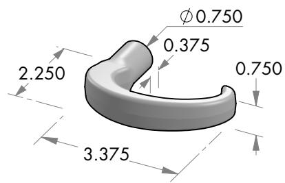
L-94 Little Hook lever.
