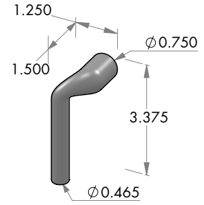
L-12OH-LH Tiny Tube lever. Left hand.
